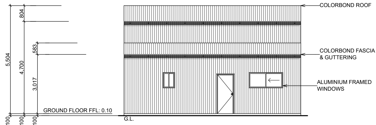
EAST ELEVATION 1:100 ALL LEVELS ASSUMED
